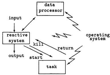
Fig. 11. Interfacing the exec primitive.
